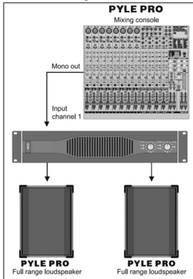
Fig .3.3 : Parallel operation
